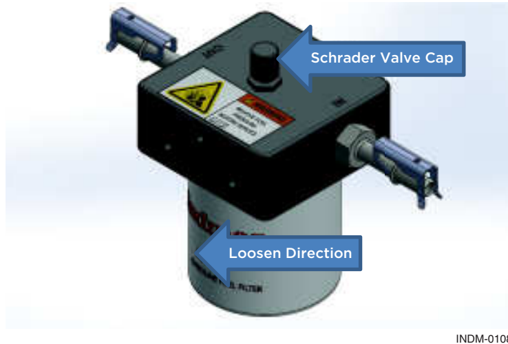
Figure 7.6 – Fuel Filter
